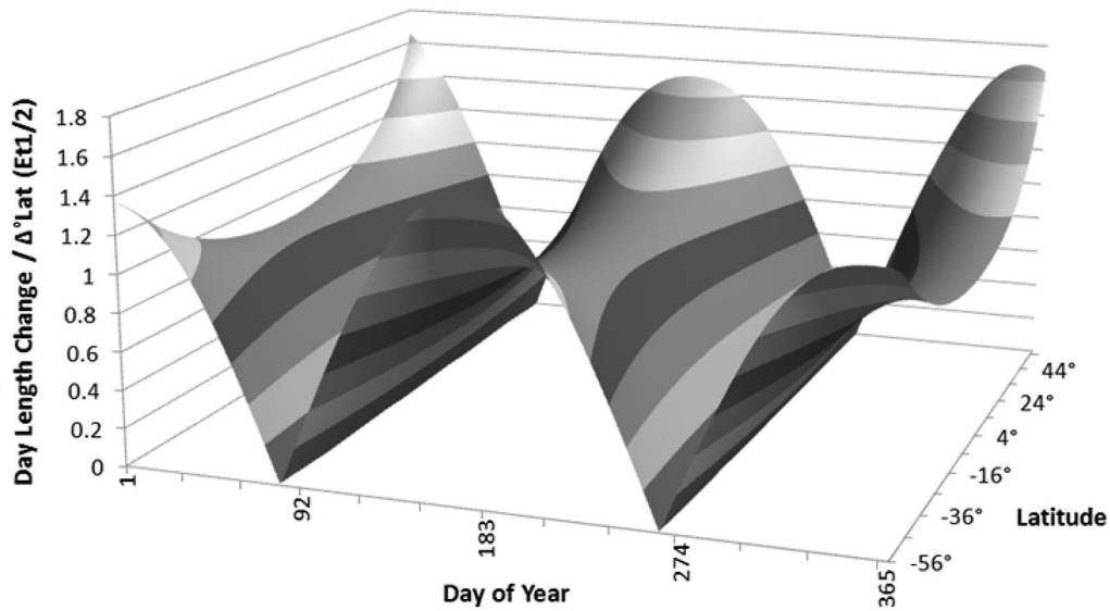
Fig. 5 Three-dimensional plot of day of day length as a function of time of year and latitudes from 56°S to 56°N. Daylight change is expressed in irradiance half-life periods ( E_{1/2} ) per Δ° of latitude. An irradiance half-life period is the time it takes for irradiance levels to double during dawn and halve during dusk. While day length around the solstices changes dramatically in the high latitudes per degree latitude travelled north or south, the dawn and dusk light gradient is also less pronounced at these latitudes. Nonetheless, day length measurement-based latitude estimates can be expected to be about 1.7 times more accurate at 56°N as compared to the equator at solstice. In conclusion, the gradients in day length are greatest during the summer and winter solstices, when the days are longest and shortest in the northern and southern hemispheres; the gradients are weakest during the fall and spring equinoxes
